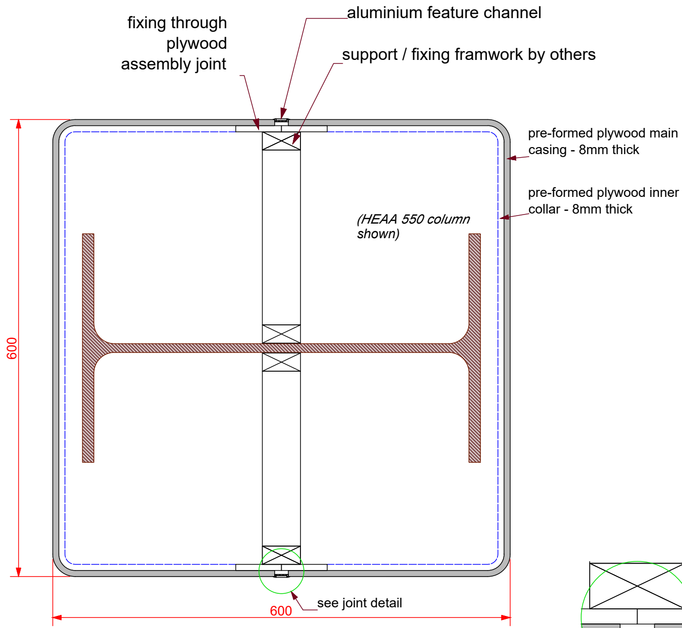
PLAN scale 1:5
