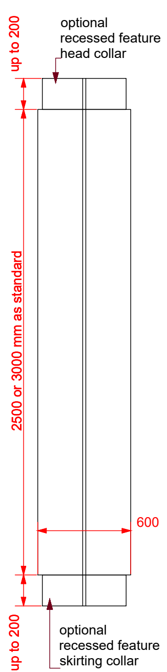
ELEVATION scale 1:25
