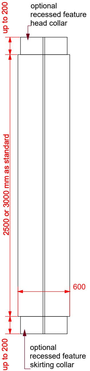
ELEVATION scale 1:25
