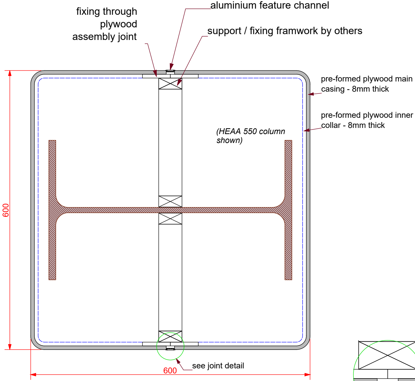
PLAN scale 1:5
