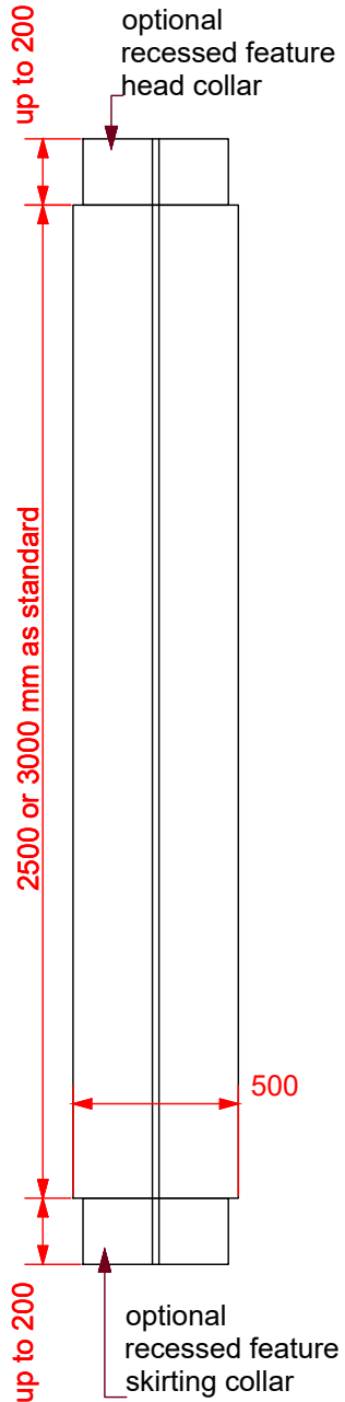
ELEVATION scale 1:25
