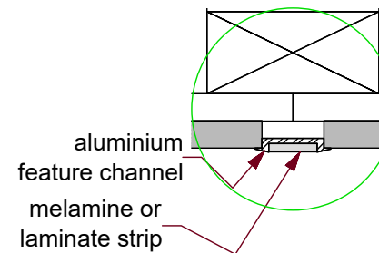
JOINT DETAIL scale 1:2
