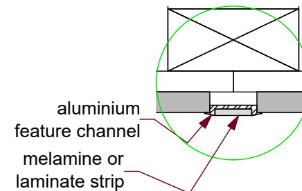
JOINT DETAIL scale 1:2
