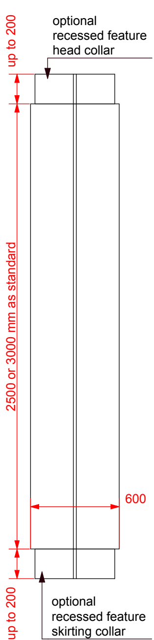
ELEVATION scale 1:25
