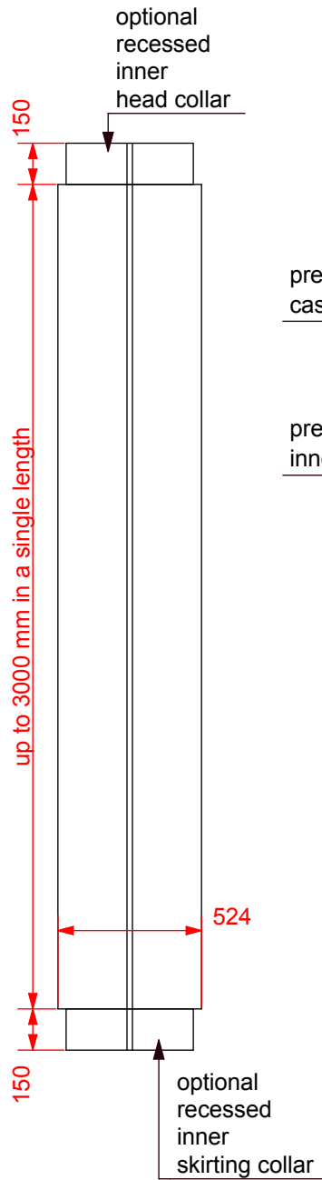
ELEVATION scale 1:25
