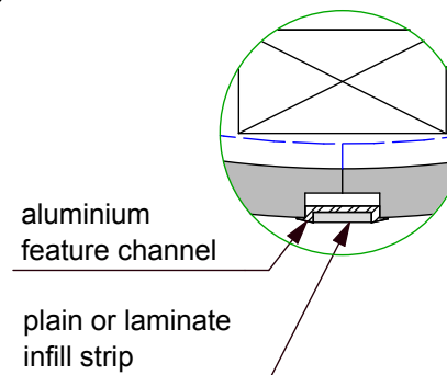
JOINT DETAIL scale 1:2
