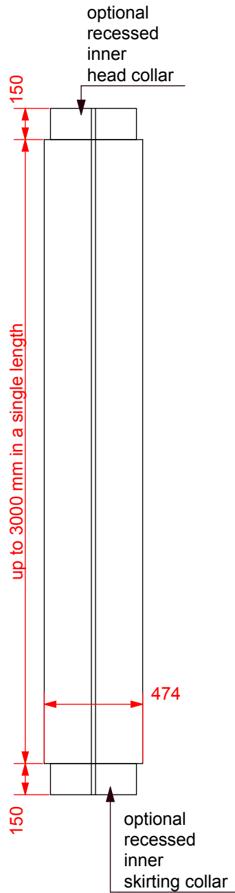
ELEVATION scale 1:25
