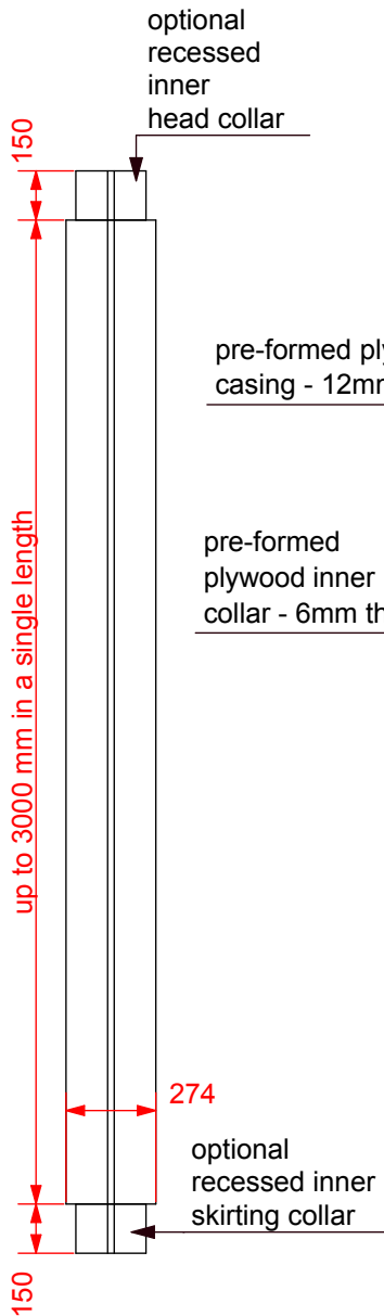
ELEVATION scale 1:25
