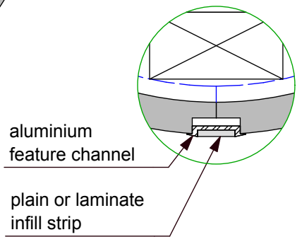
JOINT DETAIL scale 1:2
