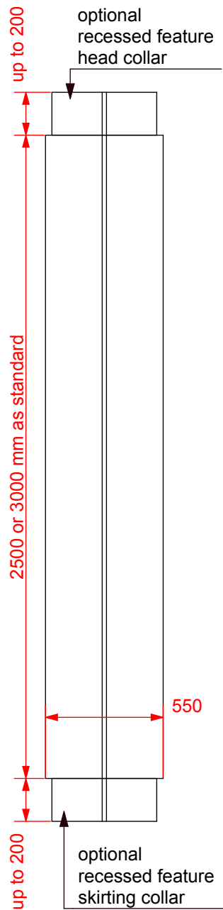
ELEVATION scale 1:25
