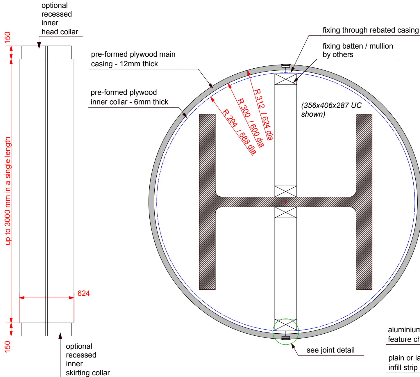
ELEVATION scale 1:25
