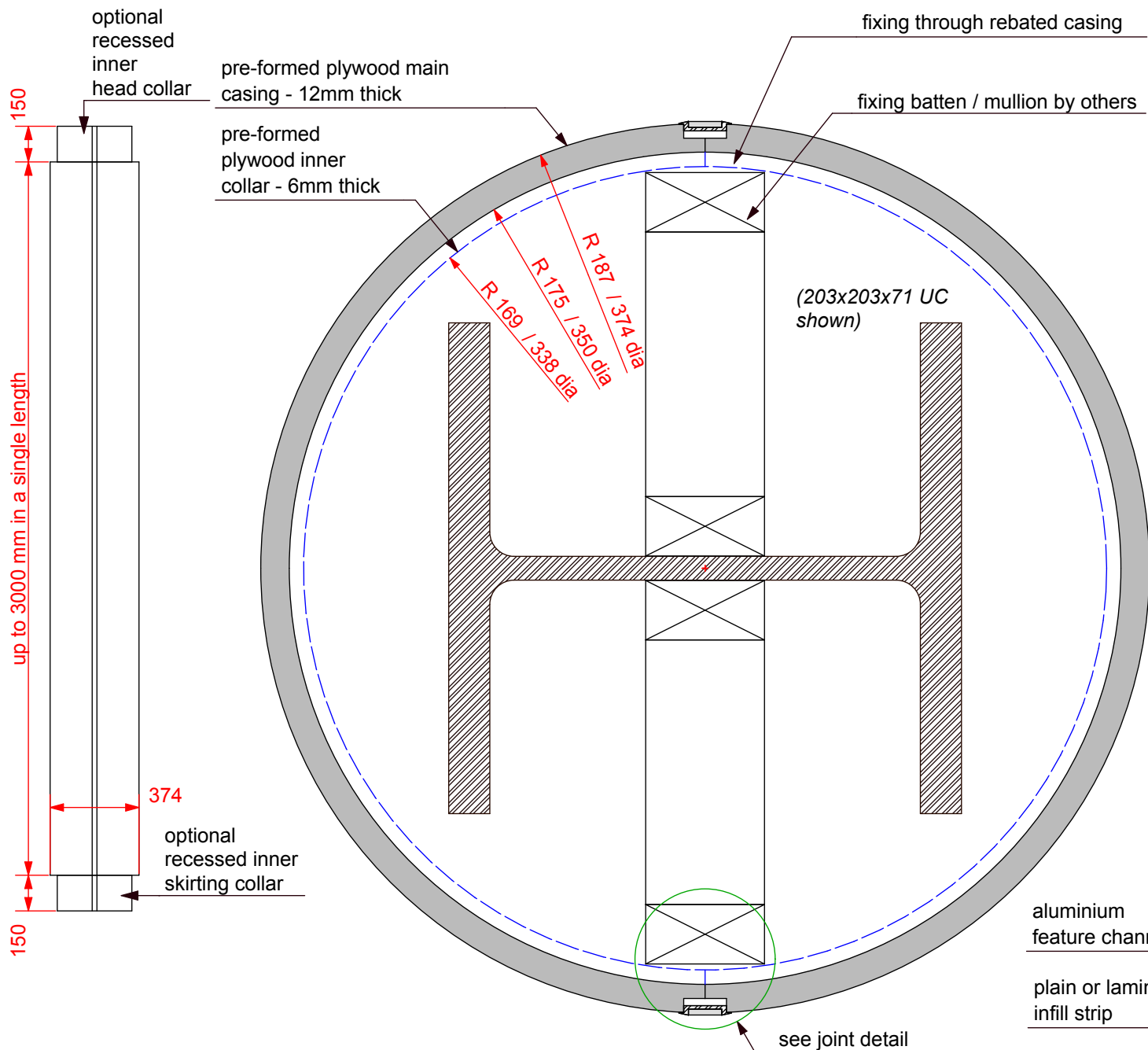
ELEVATION scale 1:25
