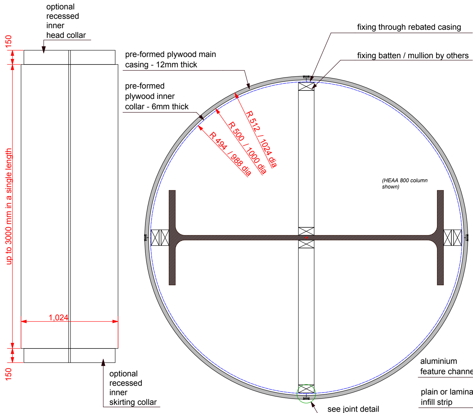
ELEVATION scale 1:25
